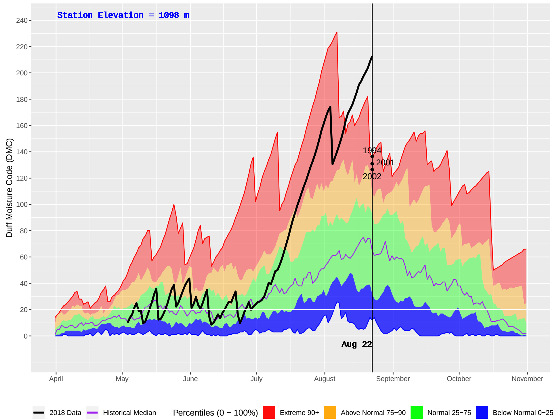
GOATFELL (401) : Historical (1986–2016) and Current (2018) Daily Duff Moisture Code (DMC)
